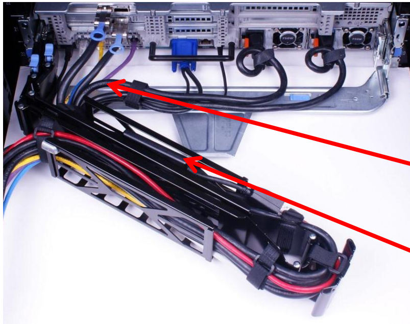
Figure 4. Routing the cables through the CMA
